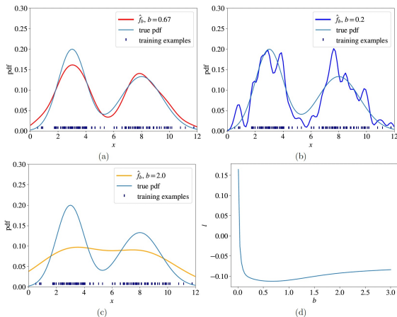
Figure 1: Kernel density estimation: (a) good fit; (b) overfitting; (c) underfitting; (d) the curve of grid search for the best value for b .
