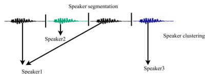
Speaker diarization
