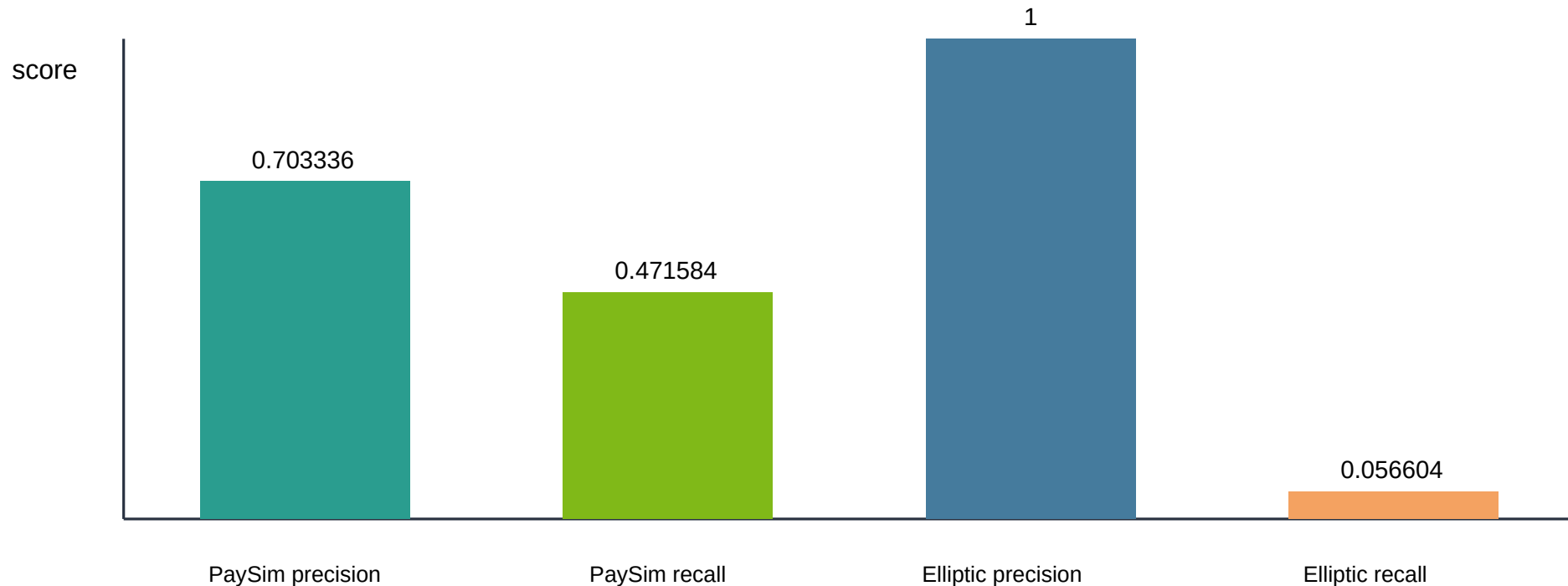
Figure 3. Review-budget precision and recall
