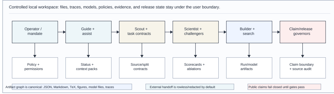
Figure 1: Local-first Relaytic agent architecture
