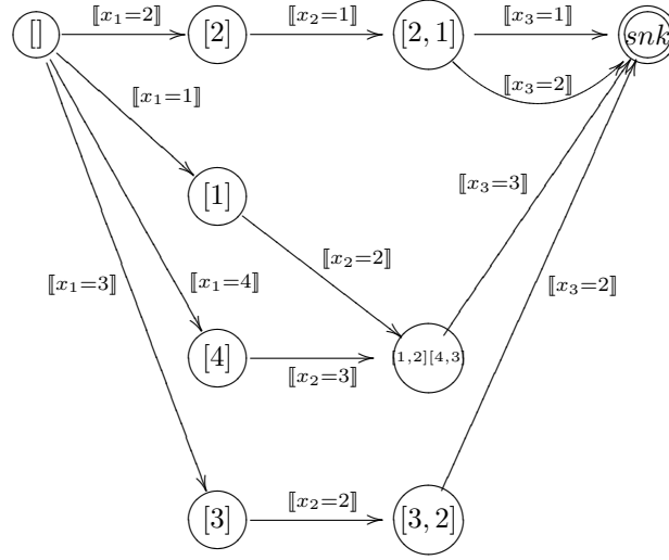
■ Figure 1 MDD encoding of Example 1.
