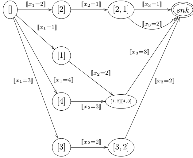
■ Figure 1 MDD encoding of ??.
