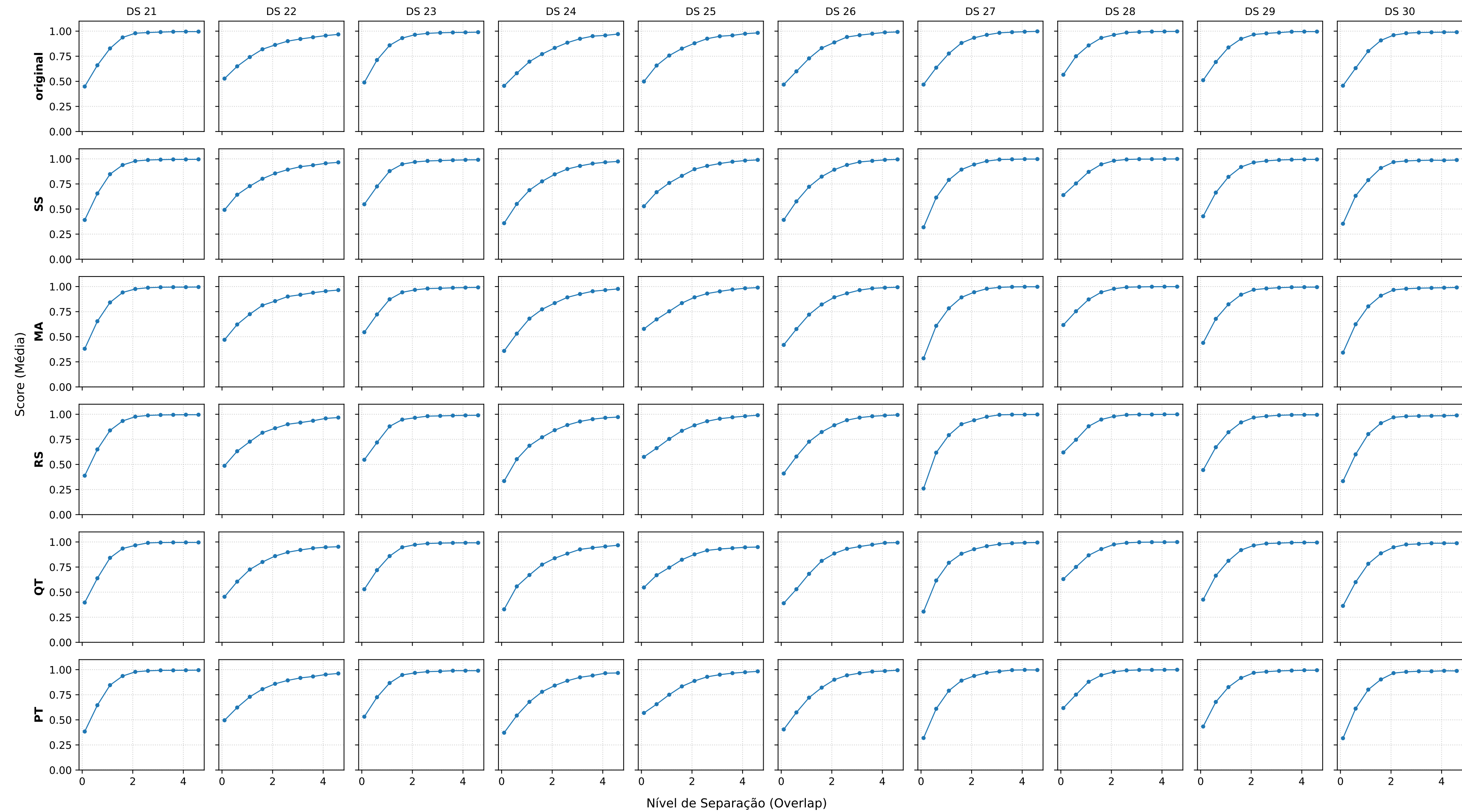
Modelo: Bagging | Métrica: F1_SCORE | Datasets: 21-30
