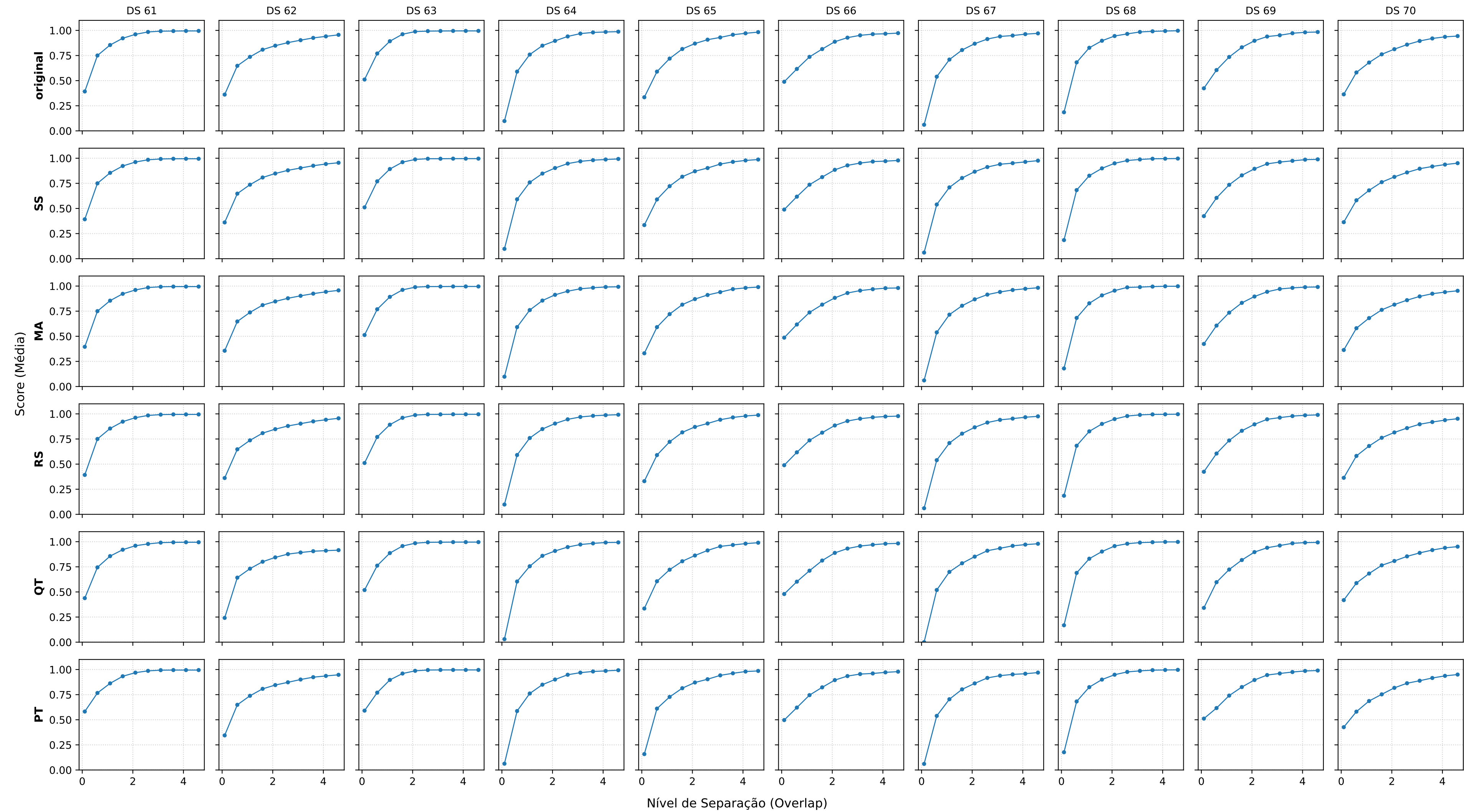
Modelo: SVM_lin | Métrica: G_MEAN | Datasets: 61-70
