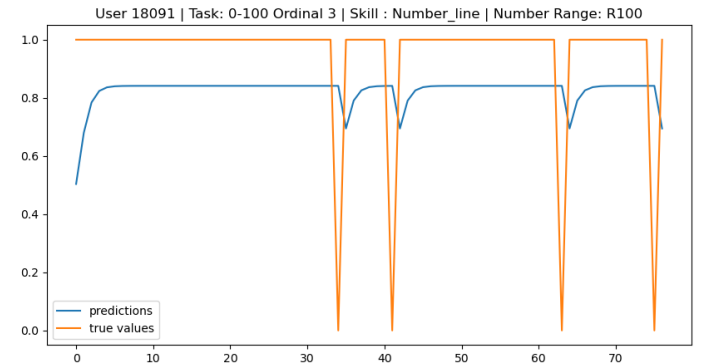
Fig. 18. Prediction of testing data of a specific user on a specific skill using the skill-id BKT model
