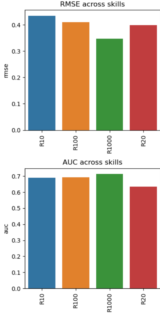
Fig. 6. Training evaluation plot for the skill-id BKT model on whole data
