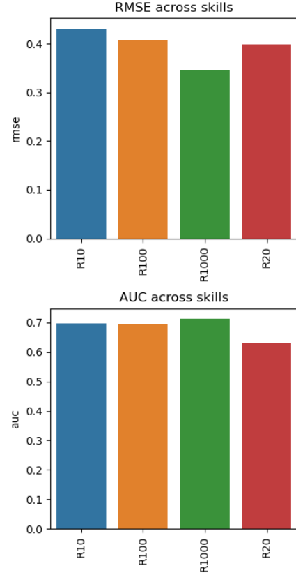
Fig. 7. Testing evaluation plot for the skill-id BKT model
