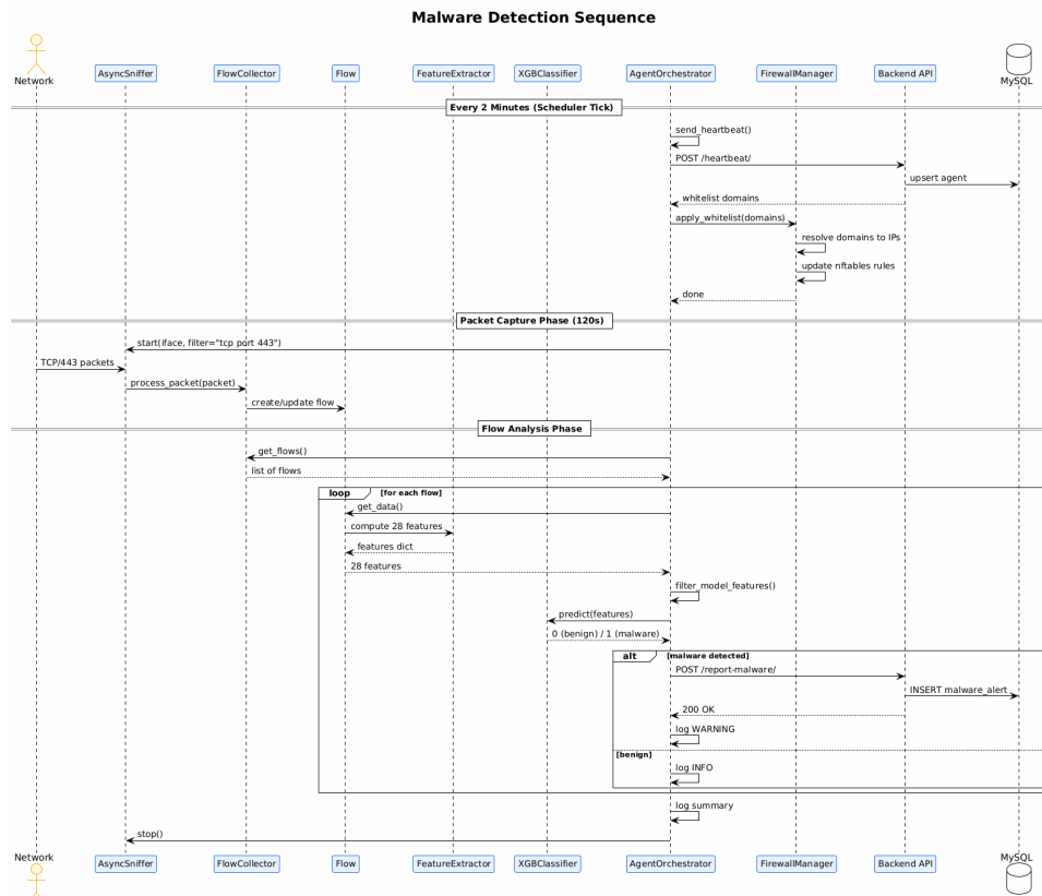
Figure 4.13: Sequence diagram of the two-layer malware detection pipeline
