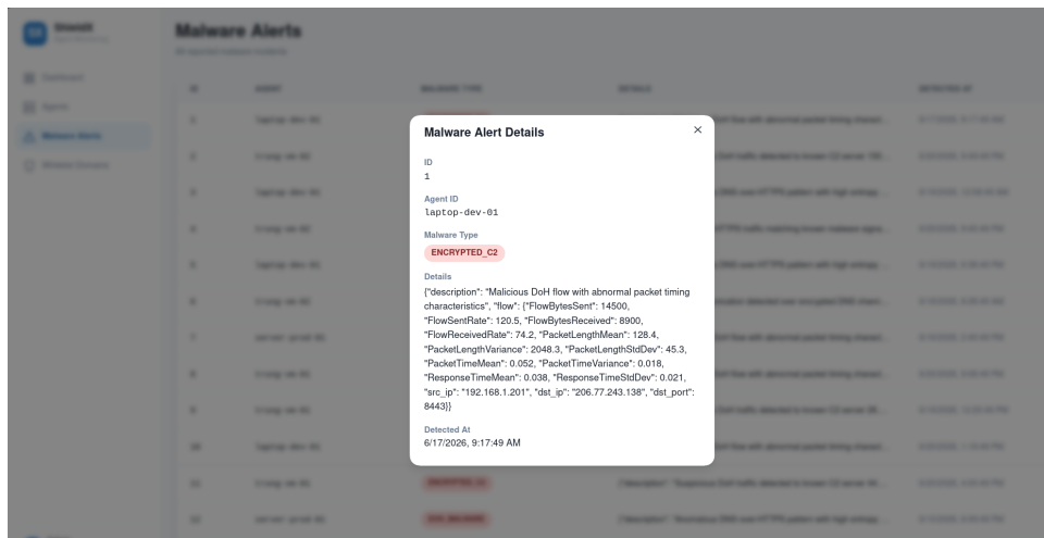
Figure 4.12: Malware alert detail modal showing full alert information on click
