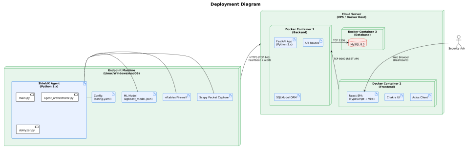
Figure 4.16: Deployment diagram of the ShieldX system
