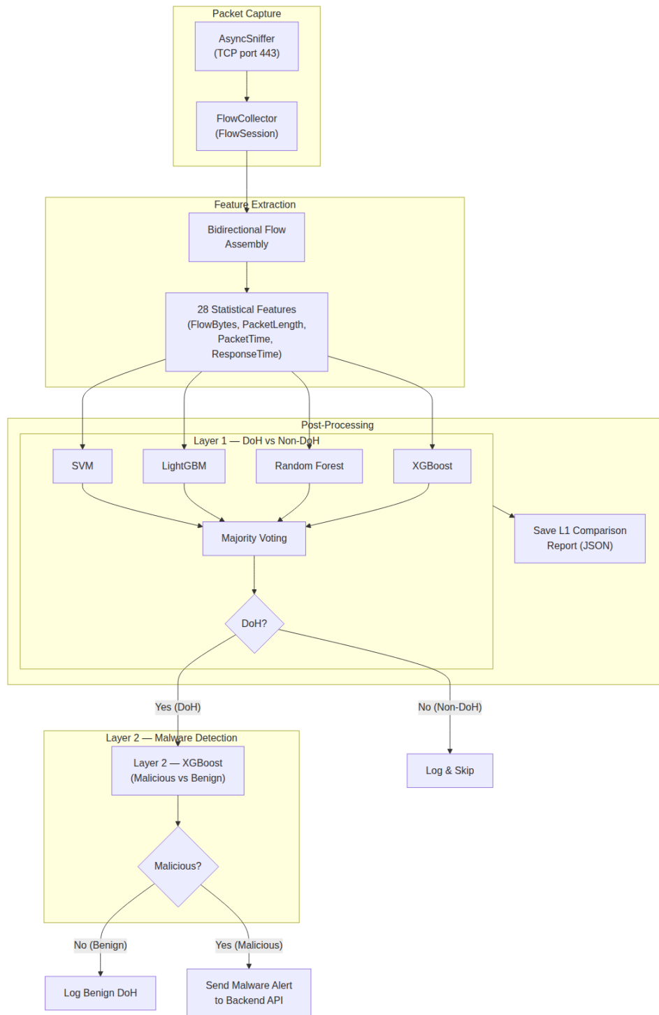
Figure 4.14: Two-layer classification pipeline: L1 ensemble (XGBoost, Random Forest, LightGBM, SVM) with majority voting for DoH detection, followed by L2 XGBoost for malware classification
