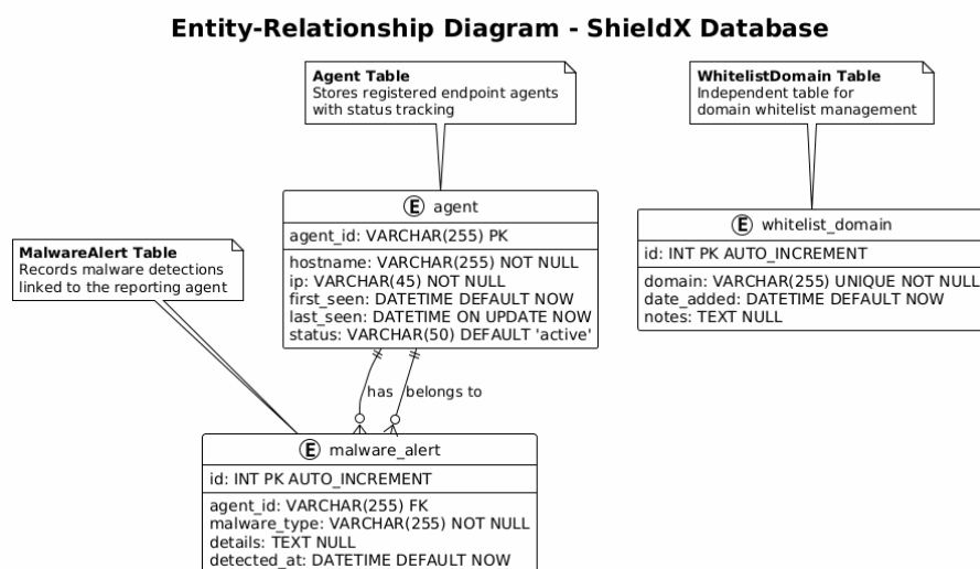
Figure 4.15: Entity-Relationship diagram of the ShieldX database
