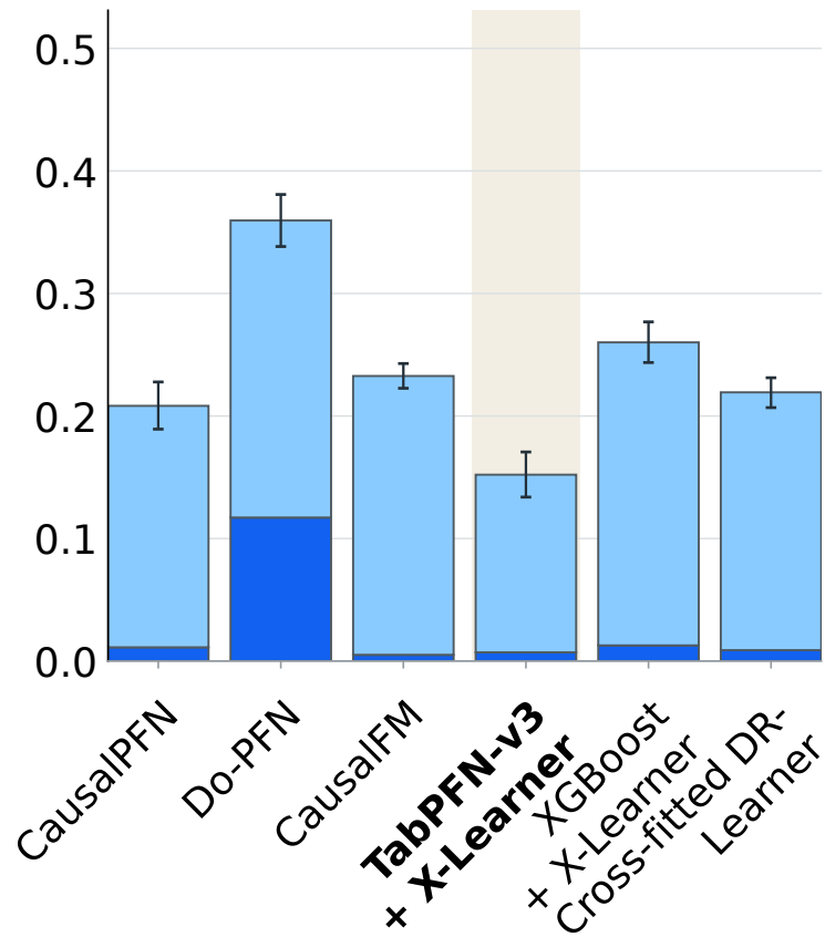
(a) Back-Door
