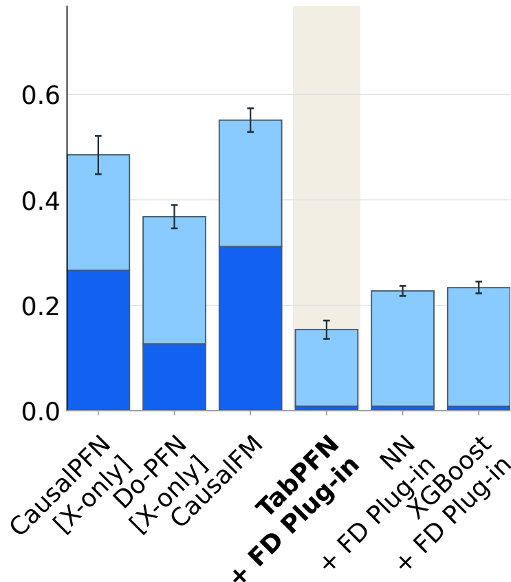
(b) Front-Door
