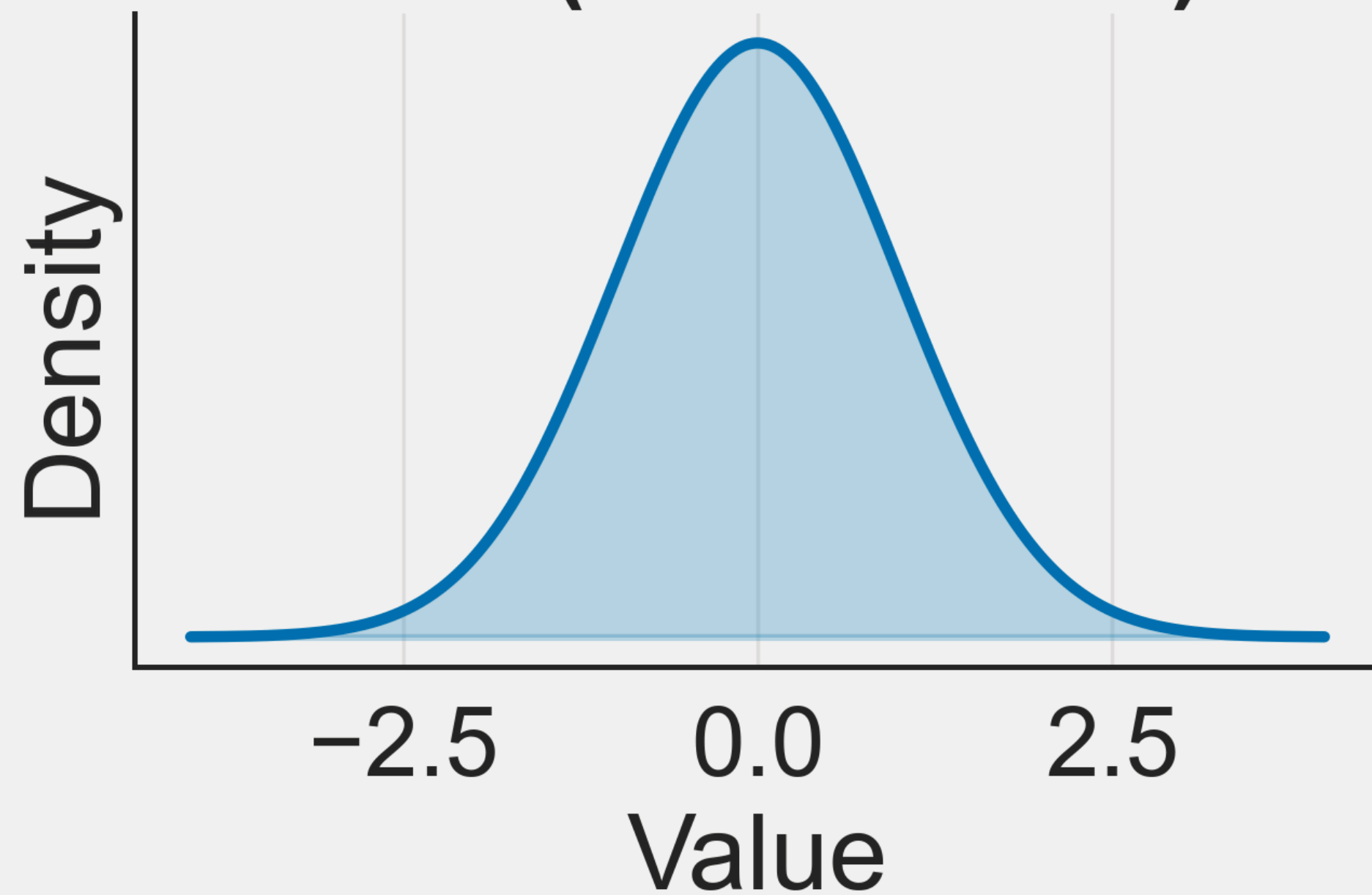
PDF (Continuous)
