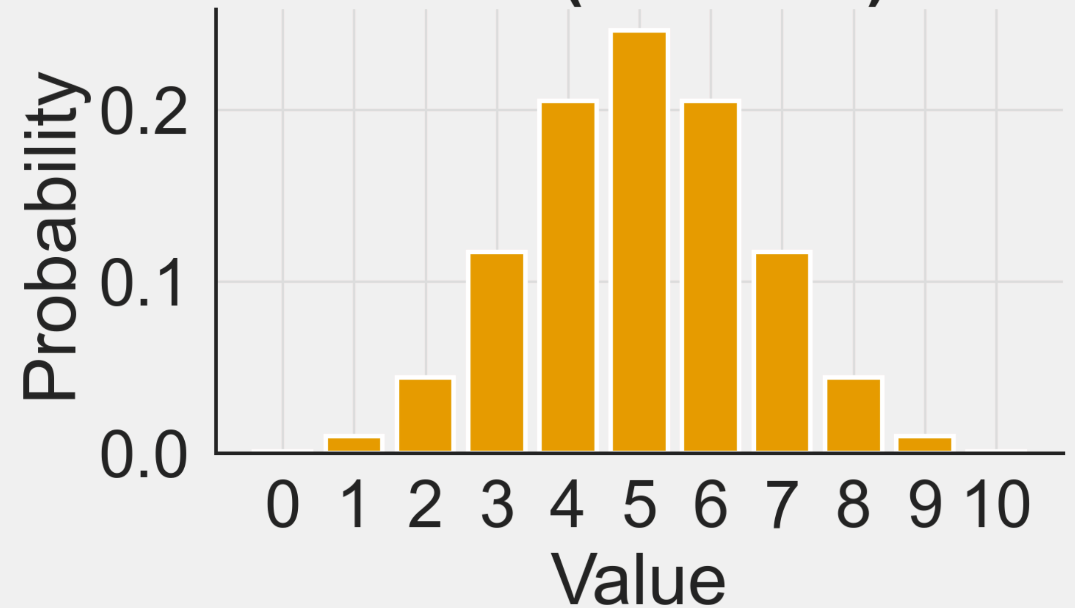
PMF (Discrete)
