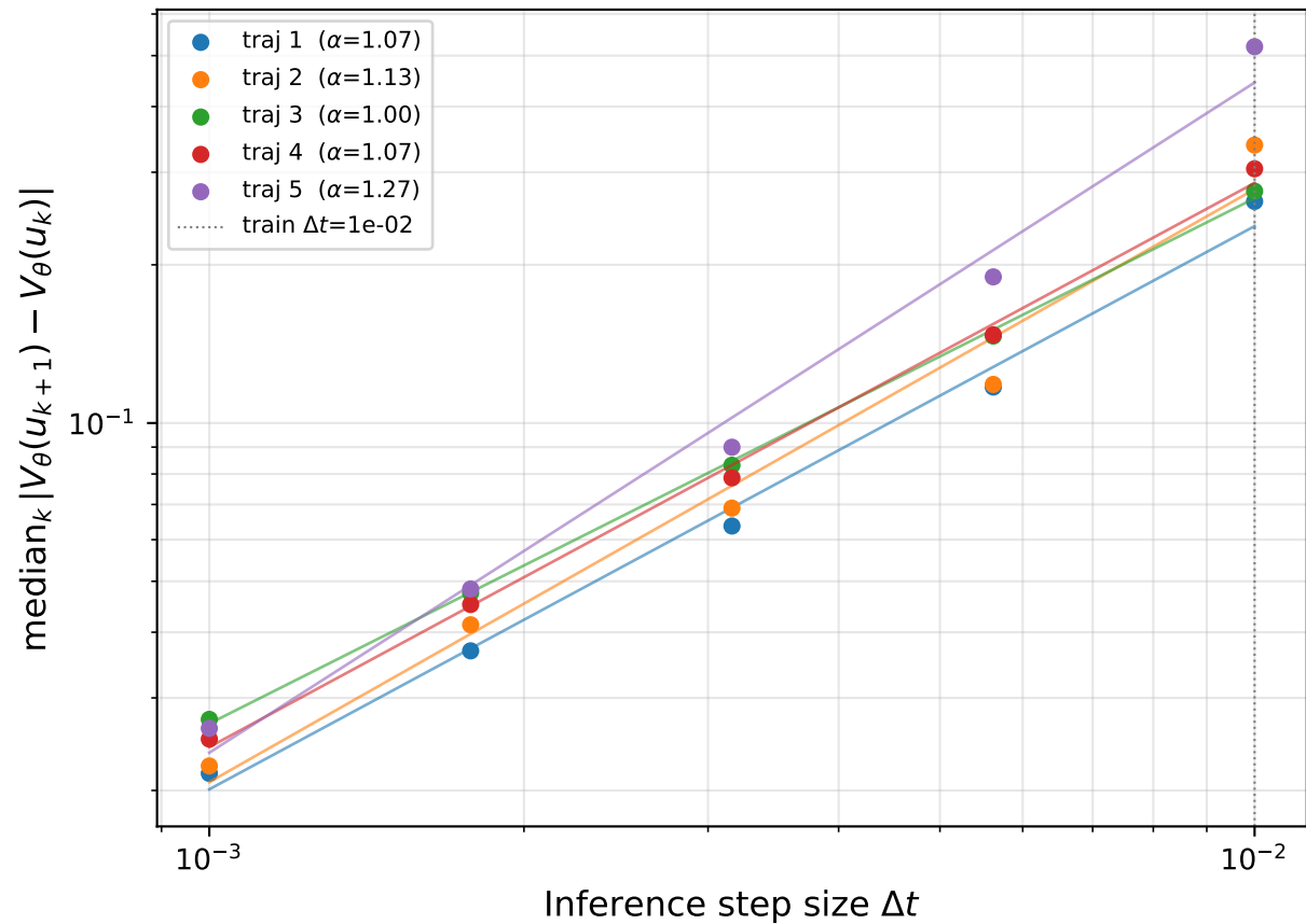
FPU chain — median one-step |\Delta V| vs \Delta t
