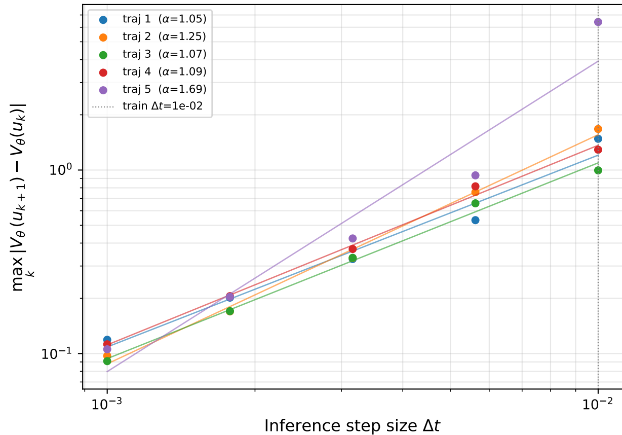
FPU chain — maximum one-step |\Delta V| vs \Delta t
