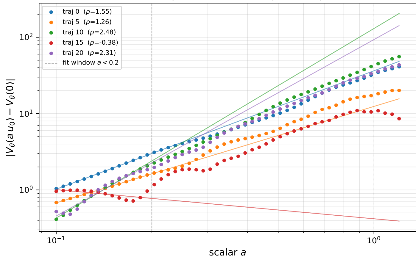
FENE — potential order via input scaling
