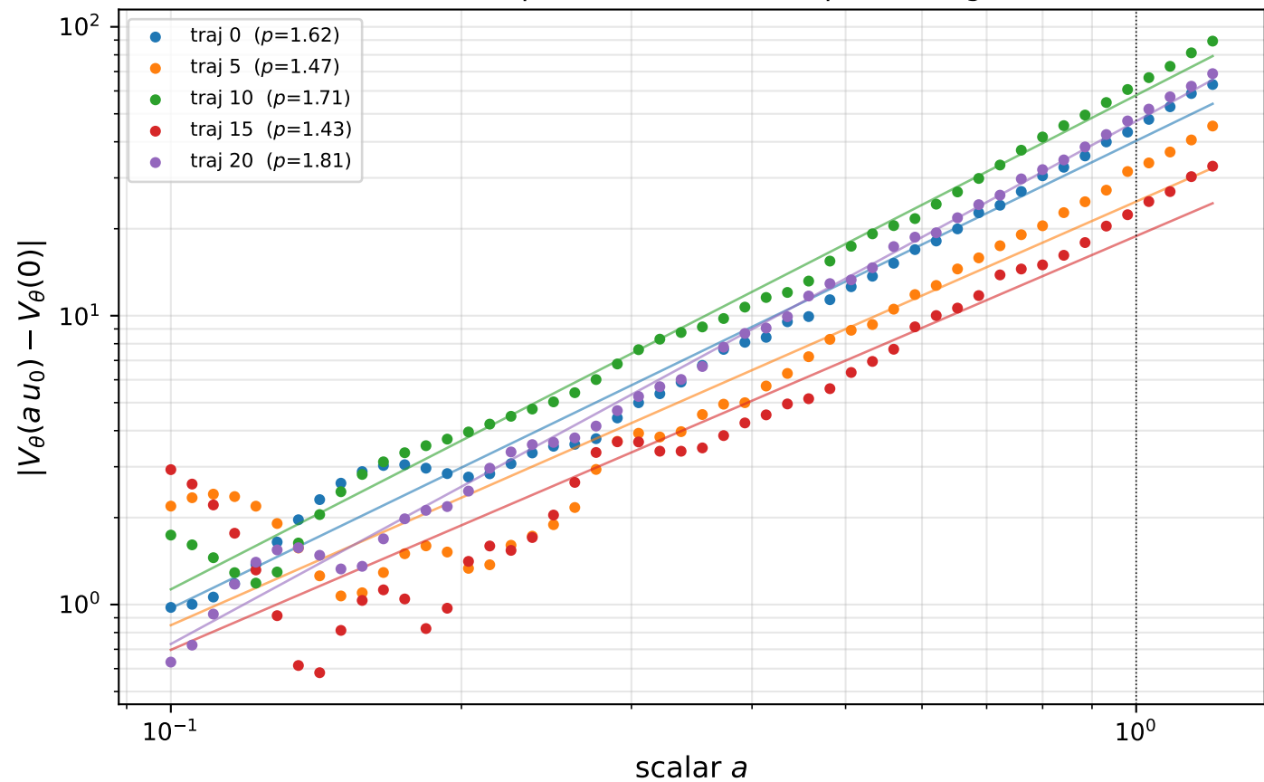
FPUT — potential order via input scaling
