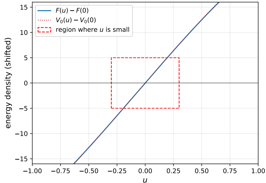
FPUT — pointwise density of V_0
