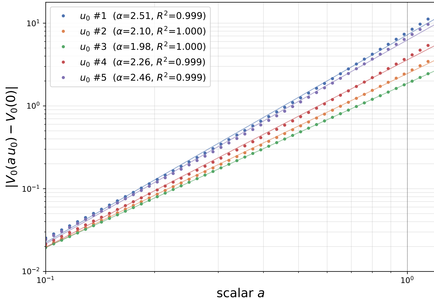
FPUT — V_0 scaling
