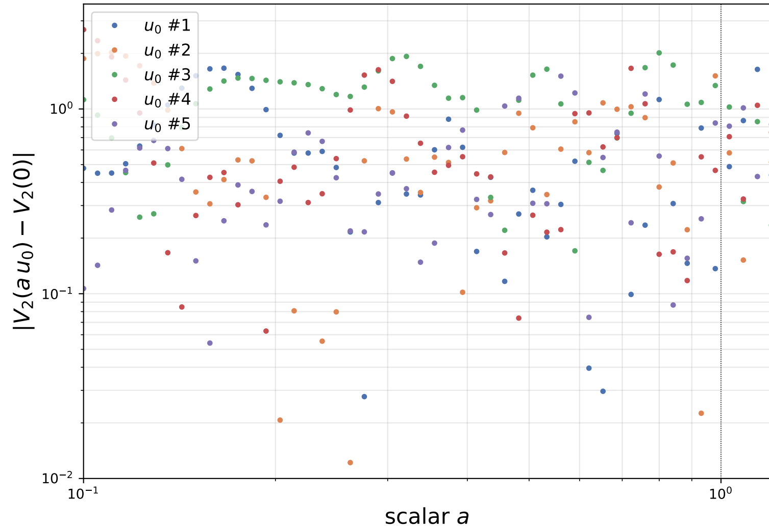
FPUT — V_2 scaling
