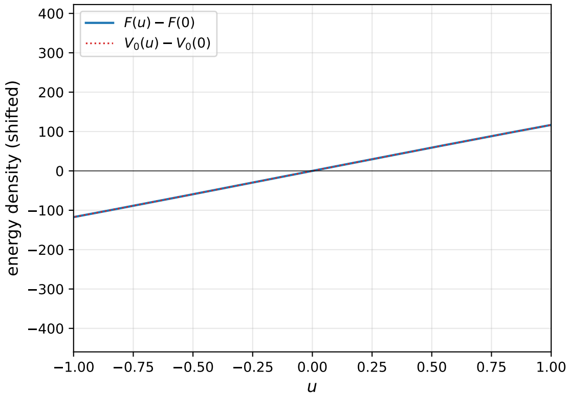
KdV — pointwise density of V_0
