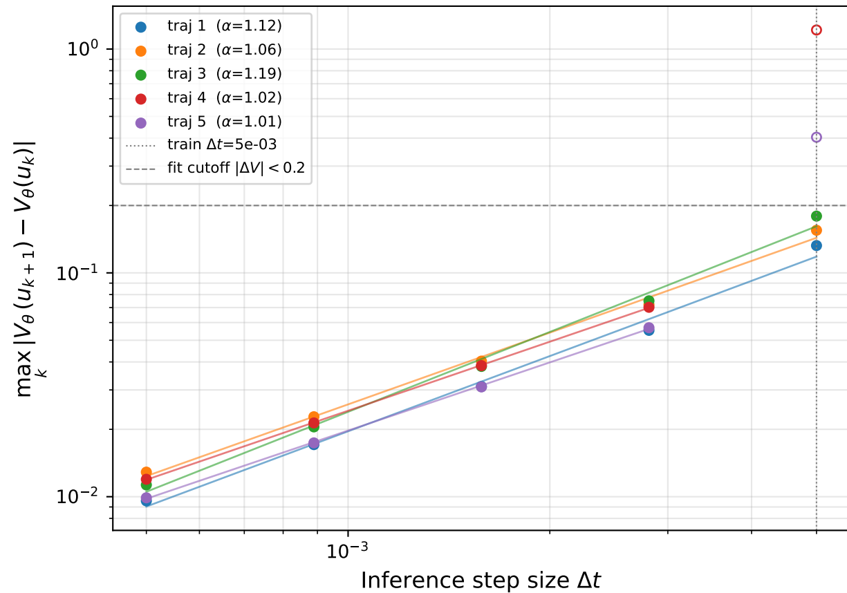
FENE chain — maximum one-step |\Delta V| vs \Delta t
