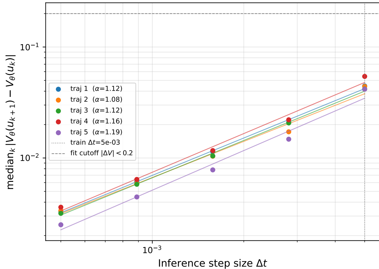
FENE chain — median one-step |\Delta V| vs \Delta t
