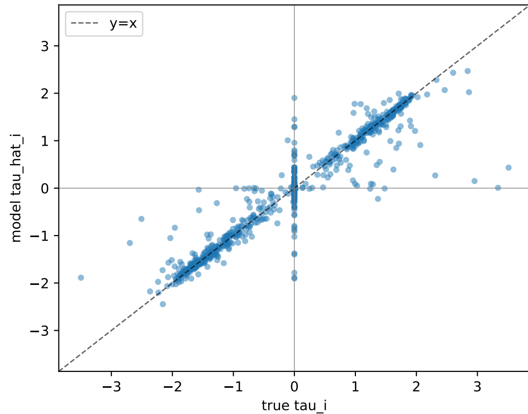
Model (Pearson = 0.947)
