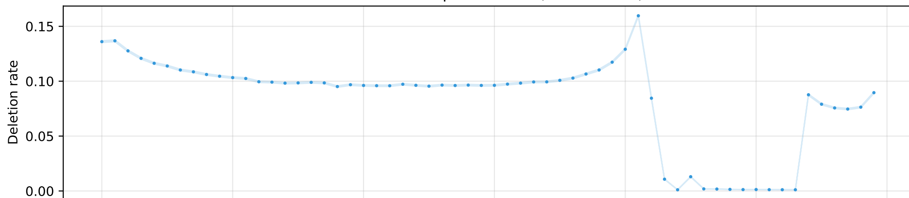
Deletion Rate per Position (with 95% CI)
