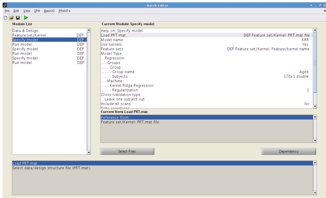
Figure 13.13: ‘Specify model’ module in the matlabbatch.
