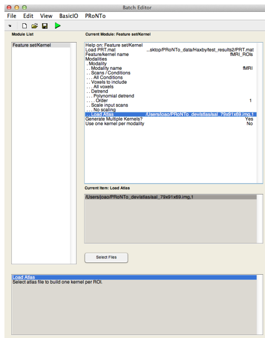
Figure 3.5: Matlabbatch GUI.
