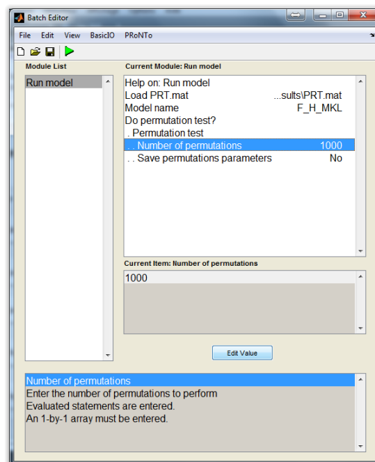
Figure 4.9: Batch interface to run a model
