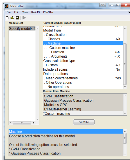
Figure 4.8: Batch interface to specify a model
