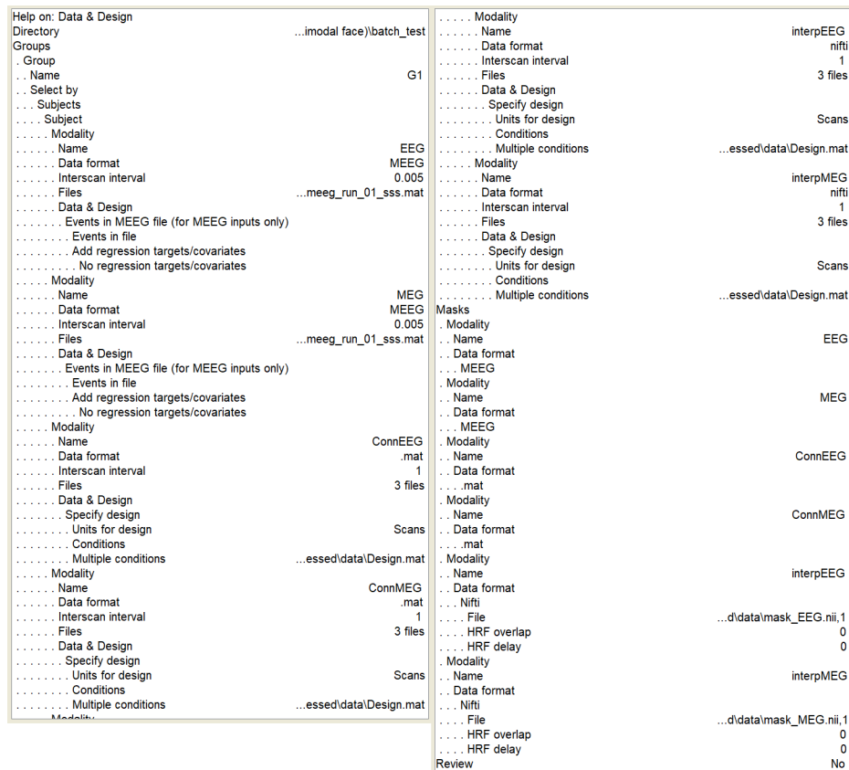
Figure 17.24: ‘Data &amp; Design’ module in matlabbatch.
