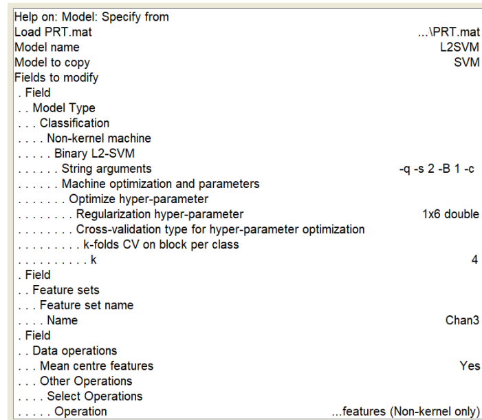
Figure 19.6: ‘Model: Specify from’ module in matlabbatch .
