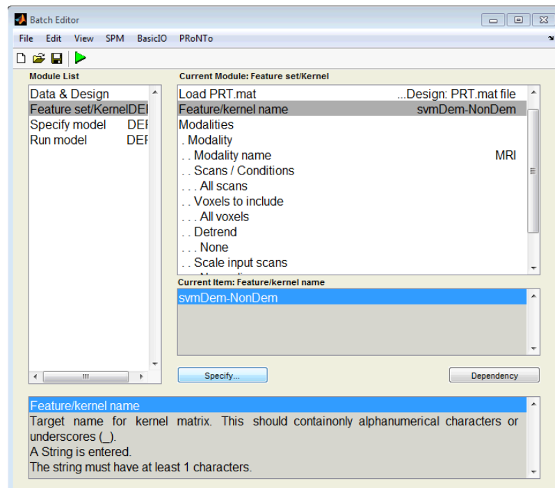
Figure 15.11: Feature set / Kernel module. Selected parameters in the Modality option.
