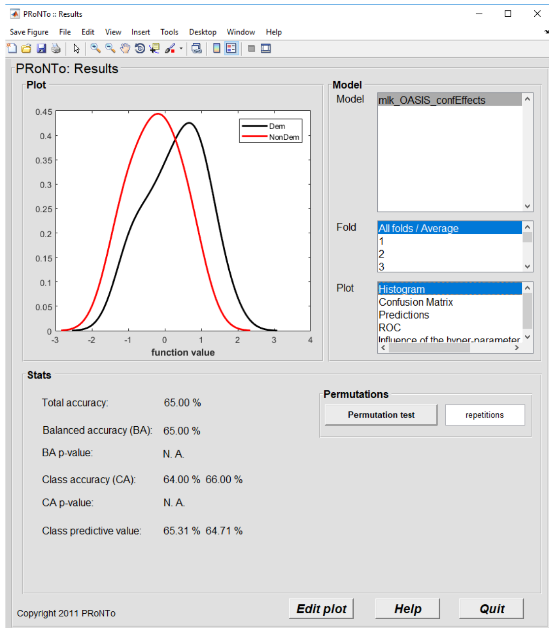
Figure 15.8: 'Accuracies of MKL without removing covariates' GUI.
