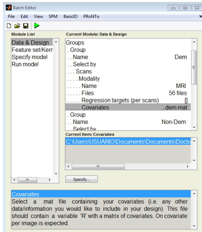
Figure 15.10: Data and design module in matlabbatch .
