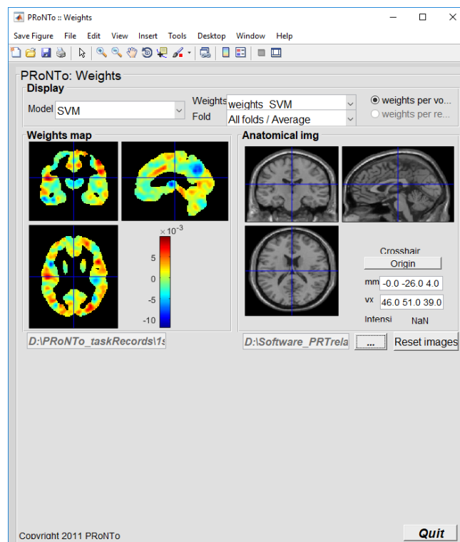
Figure 15.13: Weights map
