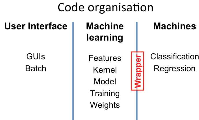
Figure 13.1: Organisation of PRoNTo's functions. From the developer's perspective the code is organised in functions and sub functions that deal with the user interface experience (such as GUI and batch functions), the core functions that implement the machine learning approaches (including extracting and preparing the features, specification and estimation of a model, cross-validation routines, etc.) and the actual machine learning algorithms (also known as machines).
