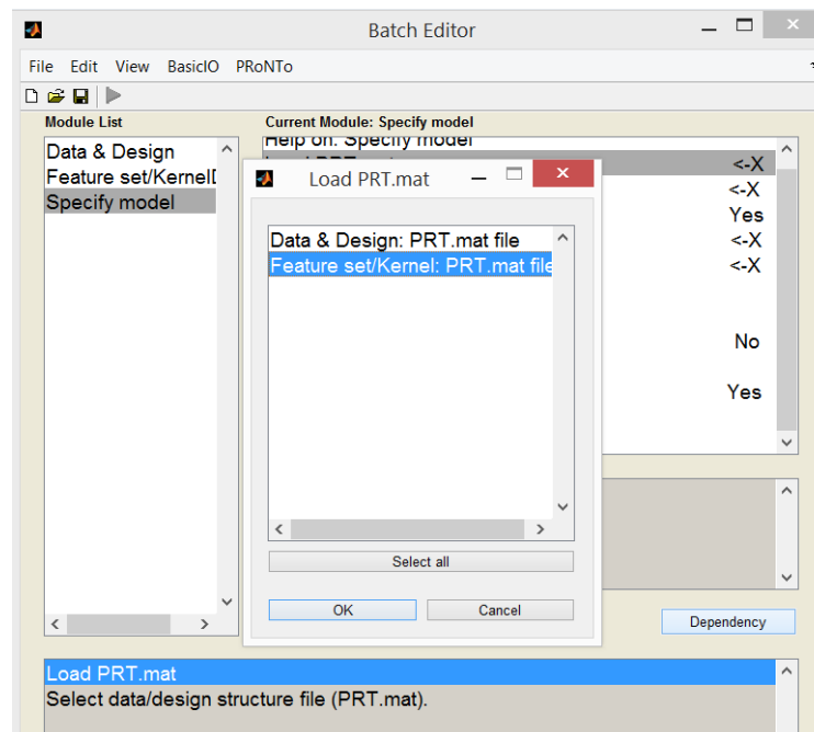
Figure 12.32: Specify model module in matlabbatch . This window is called to establish a dependency connection with the previous ‘Feature set / Kernel’ module.
