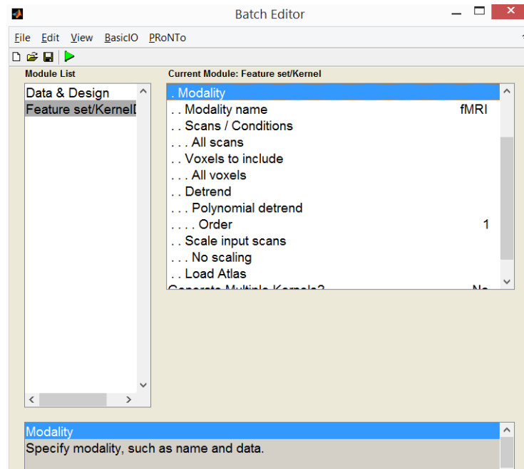
Figure 12.30: Feature set / Kernel module. Selected parameters in the Modality option.
