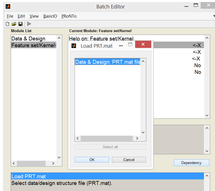
Figure 12.29: Feature set / Kernel module in matlabbatch . This window is called to establish a dependency connection with the previous ‘Data and design’ module.
