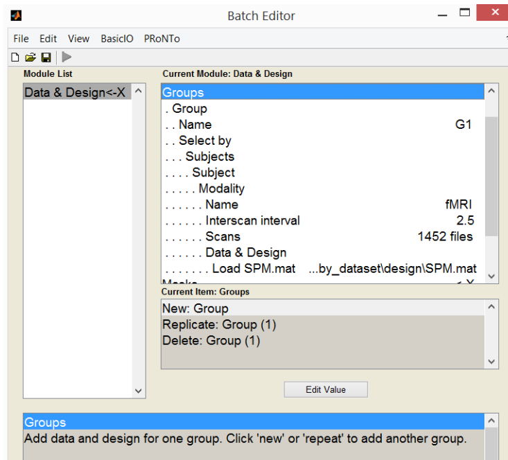
Figure 12.26: Data and design module in matlabbatch .
