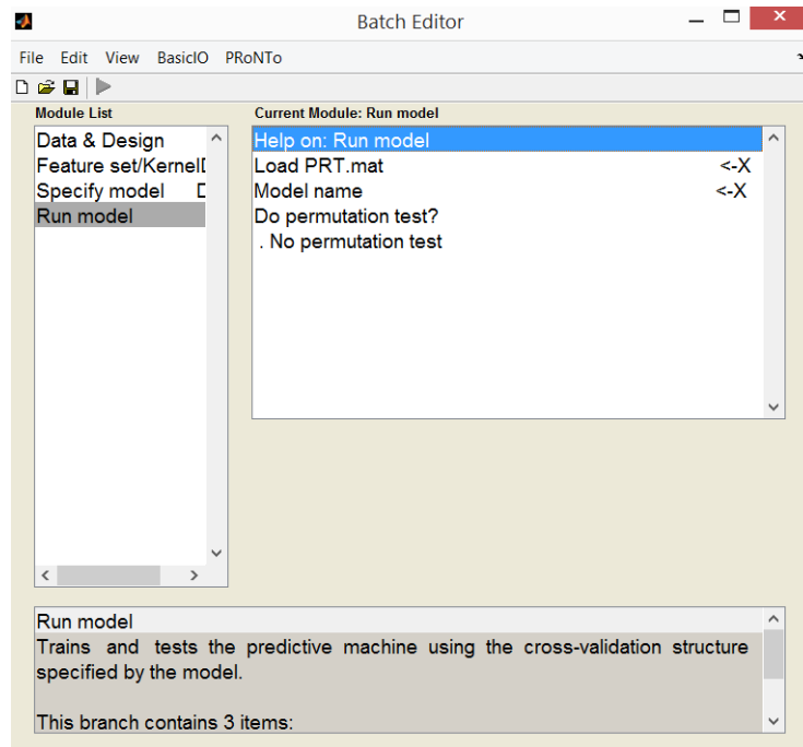
Figure 12.34: Run model module in matlabbatch .
