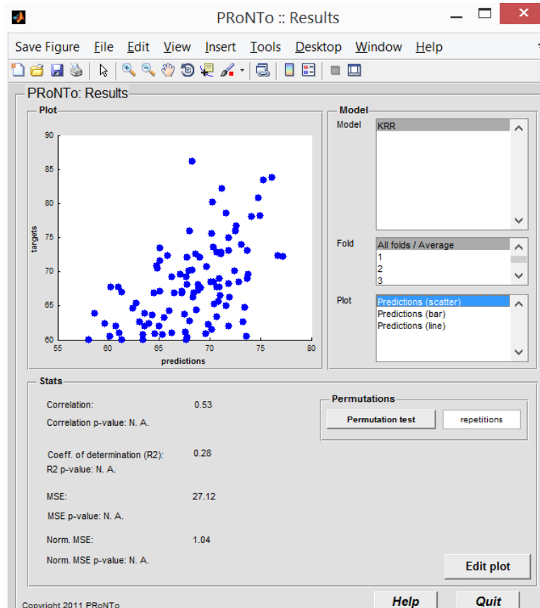
Figure 13.6: 'Results' GUI.
