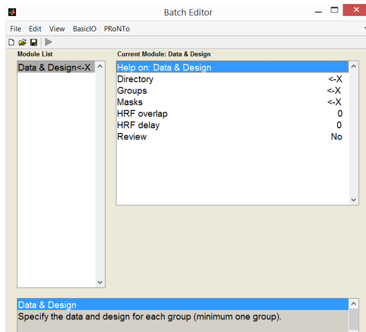
Figure 14.10: Data and design module in matlabbatch .
