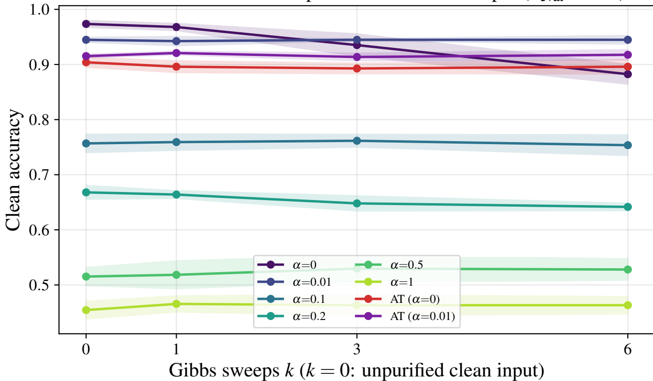
d3r10c64 — cost of Gibbs purification on clean input ( n_{\text{eval}} = 250 )
