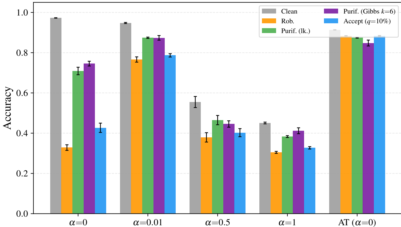
d3r10c64 — defenses at \epsilon = 0.05
