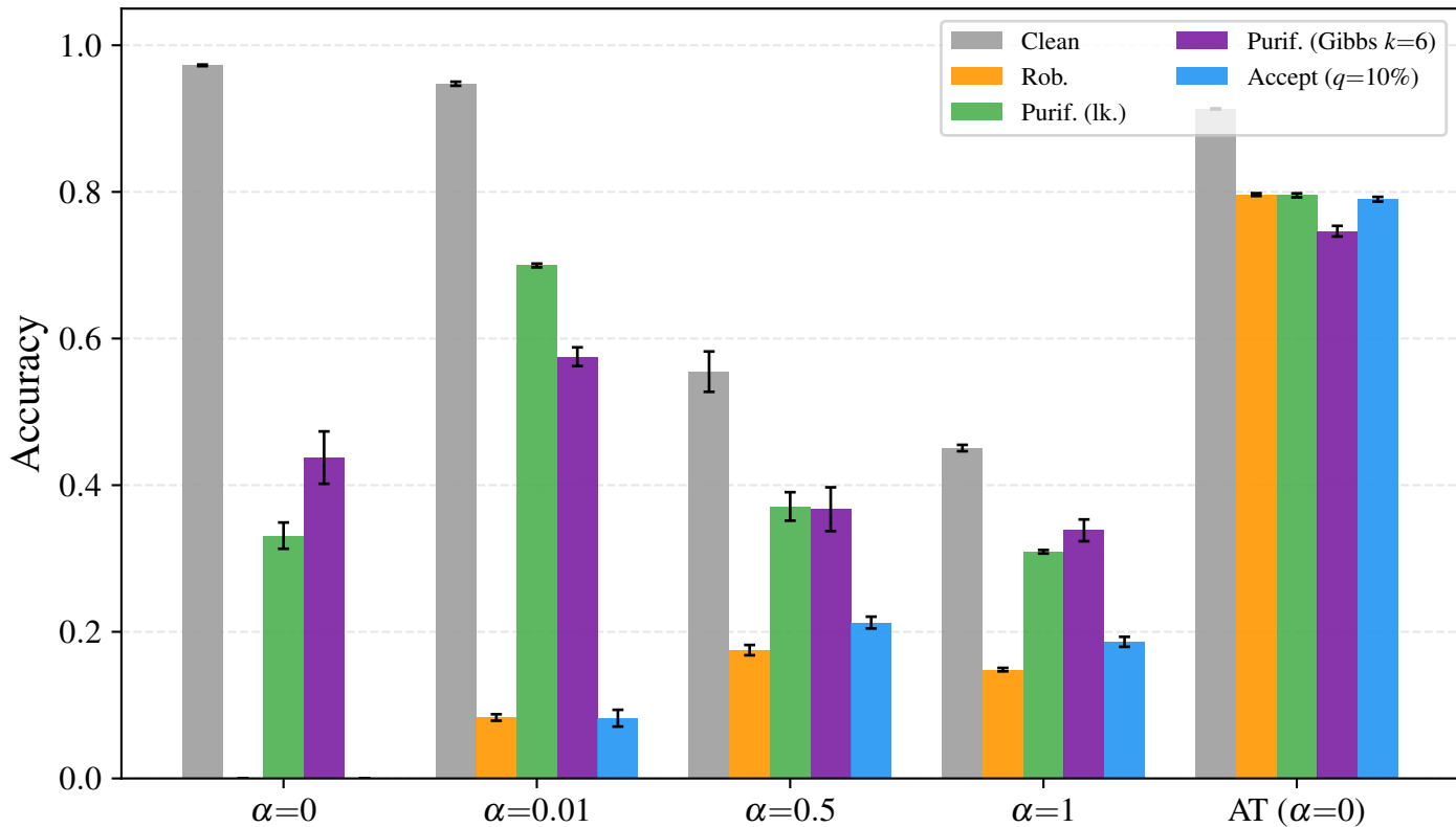
d3r10c64 — defenses at \epsilon = 0.15
