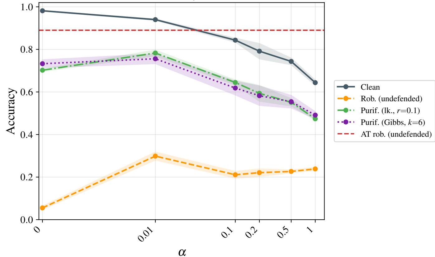
d3r40c64 — accuracy vs \alpha ( \epsilon = 0.1 )
