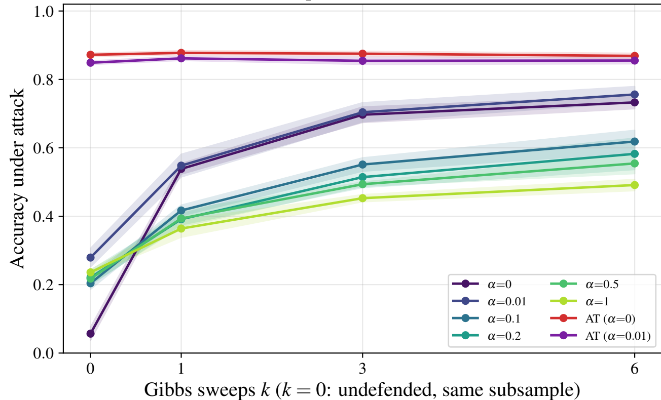
d3r40c64 — Gibbs purification ( \varepsilon = 0.1 , n_{\text{eval}} = 250 )
