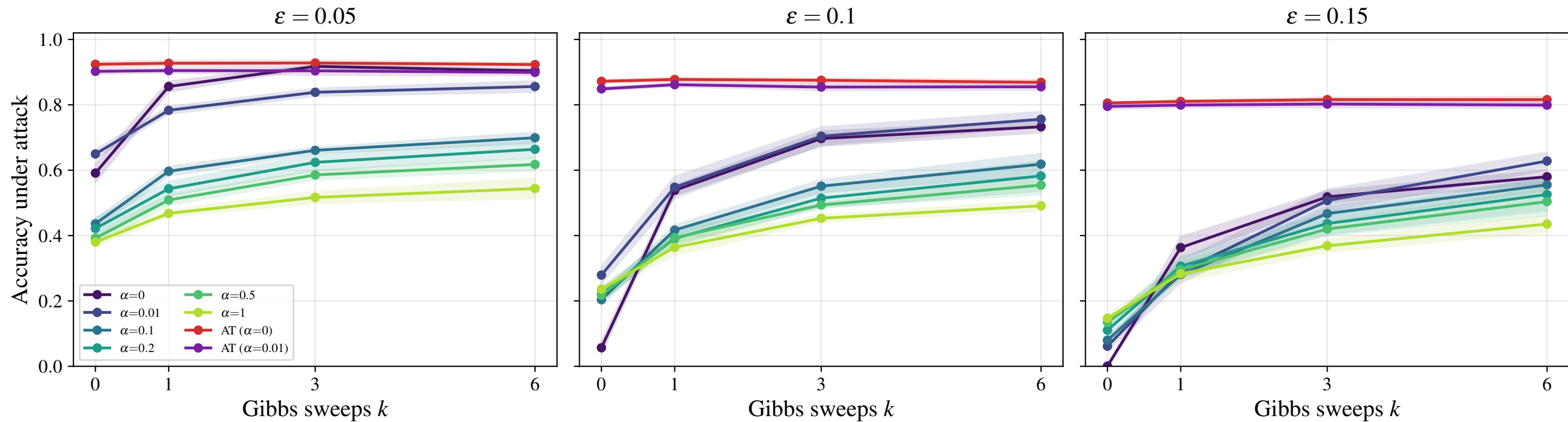
d3r40c64 — Gibbs purification vs k ( n_{\text{eval}} = 250 )
