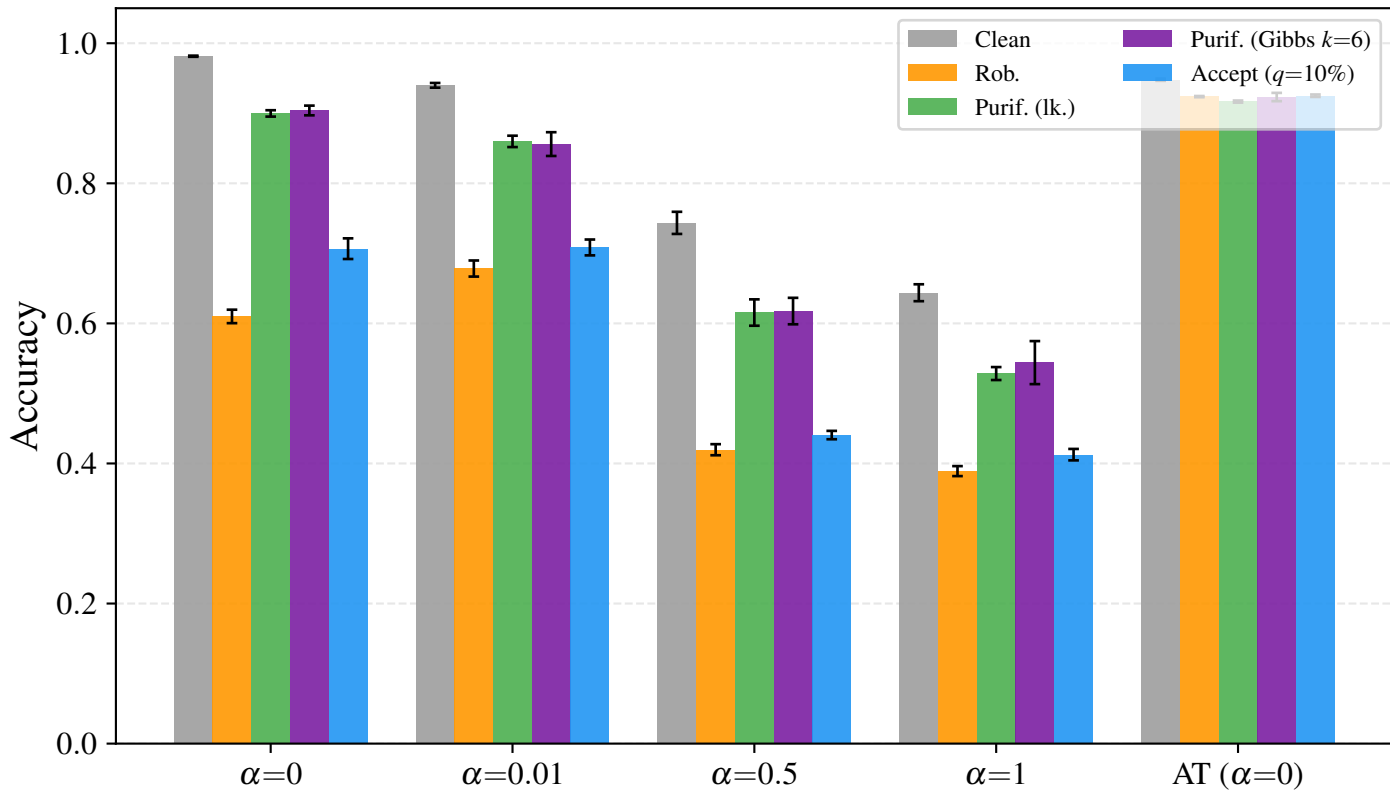
d3r40c64 — defenses at \epsilon = 0.05
