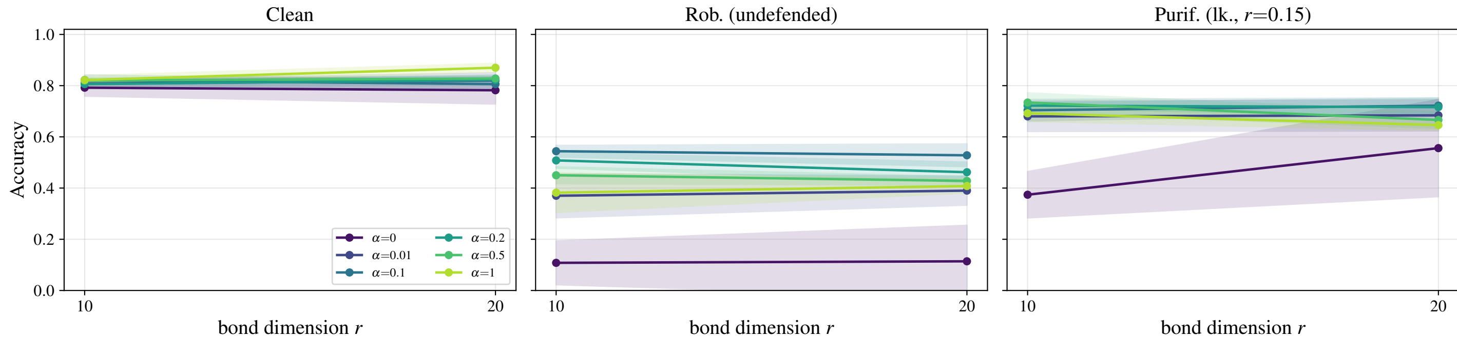
ecg200 — metrics vs bond dimension ( \varepsilon = 0.1 )
