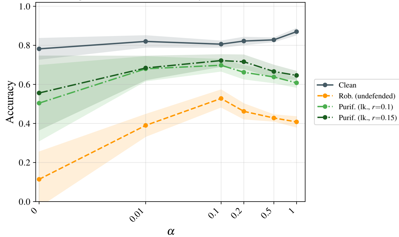
ecg200 d3r20c64 — accuracy vs \alpha ( \varepsilon = 0.1 )
