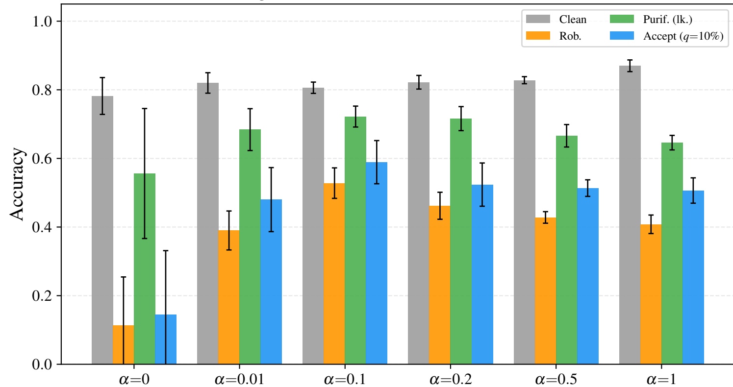
ecg200 d3r20c64 — defenses at \epsilon = 0.1
