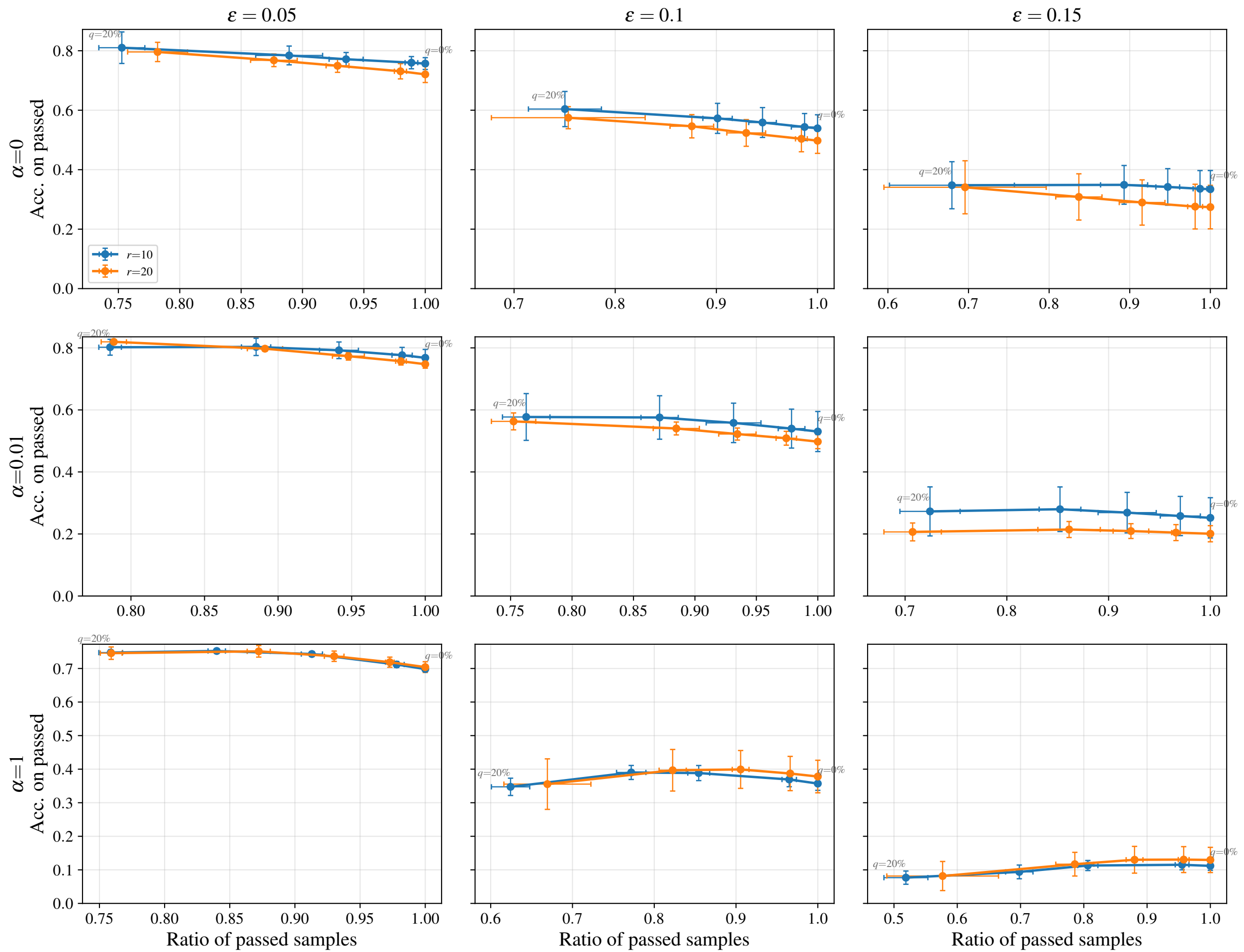
italypowerdemand — detection operating curve by bond dimension
