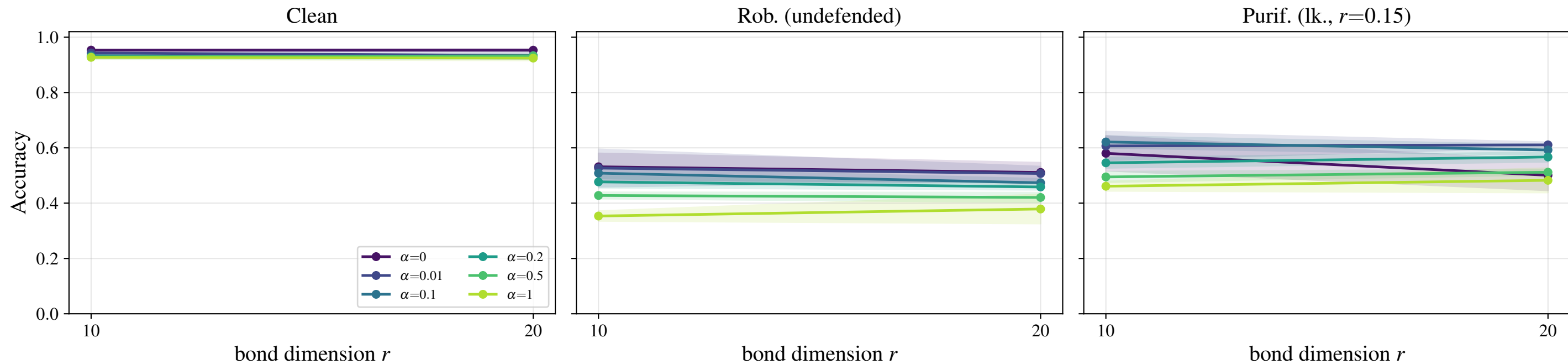
italypowerdemand — metrics vs bond dimension ( \varepsilon = 0.1 )
