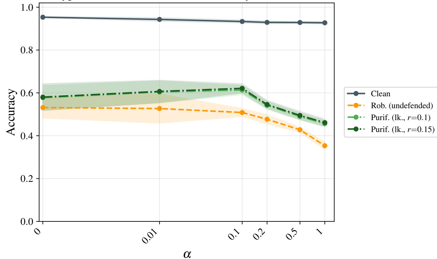
italypowerdemand d3r10c64 — accuracy vs \alpha ( \epsilon = 0.1 )
