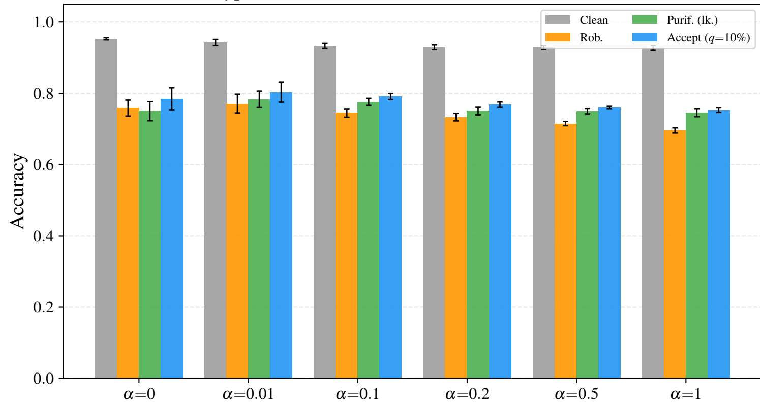
italypowerdemand d3r10c64 — defenses at \varepsilon = 0.05
