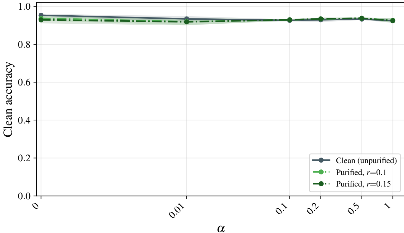
italypowerdemand d3r20c64 — cost of purification on clean input
