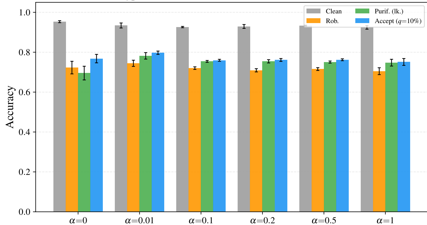
italypowerdemand d3r20c64 — defenses at \varepsilon = 0.05
