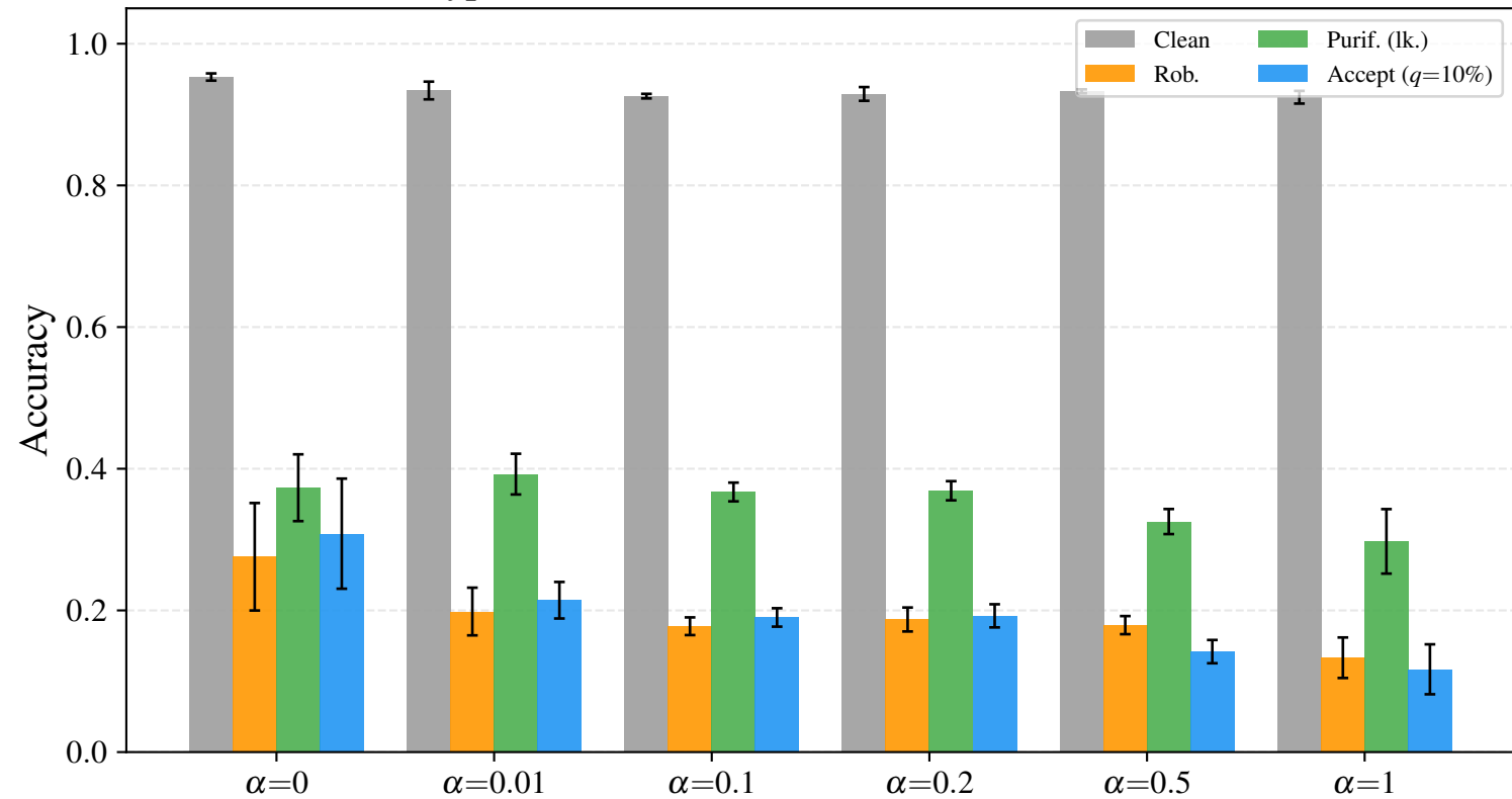
italypowerdemand d3r20c64 — defenses at \varepsilon = 0.15
