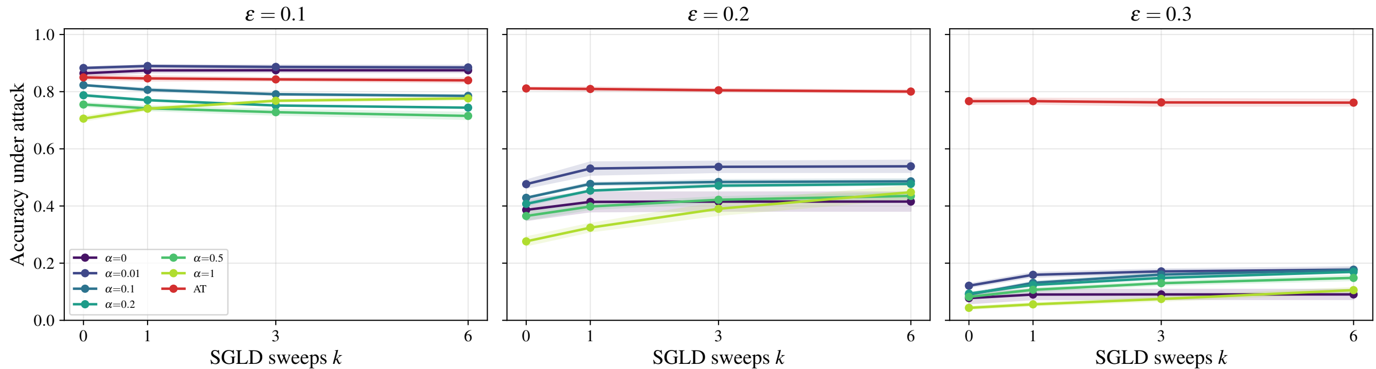
JEM — SGLD purification vs k ( n_{eval} = 1000 )
