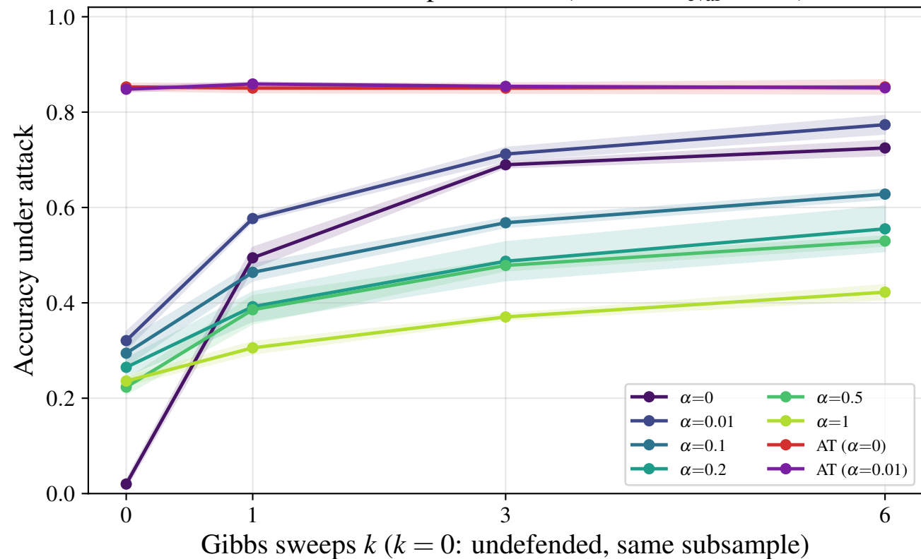
d3r20c64 — Gibbs purification ( \varepsilon = 0.1 , n_{\text{eval}} = 250 )
