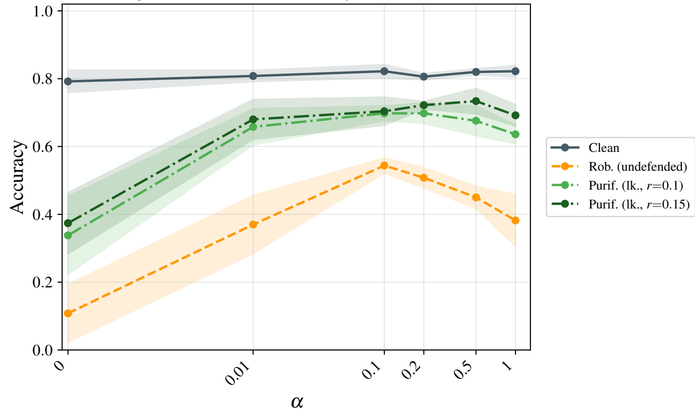
ecg200 d3r10c64 — accuracy vs \alpha ( \epsilon = 0.1 )
