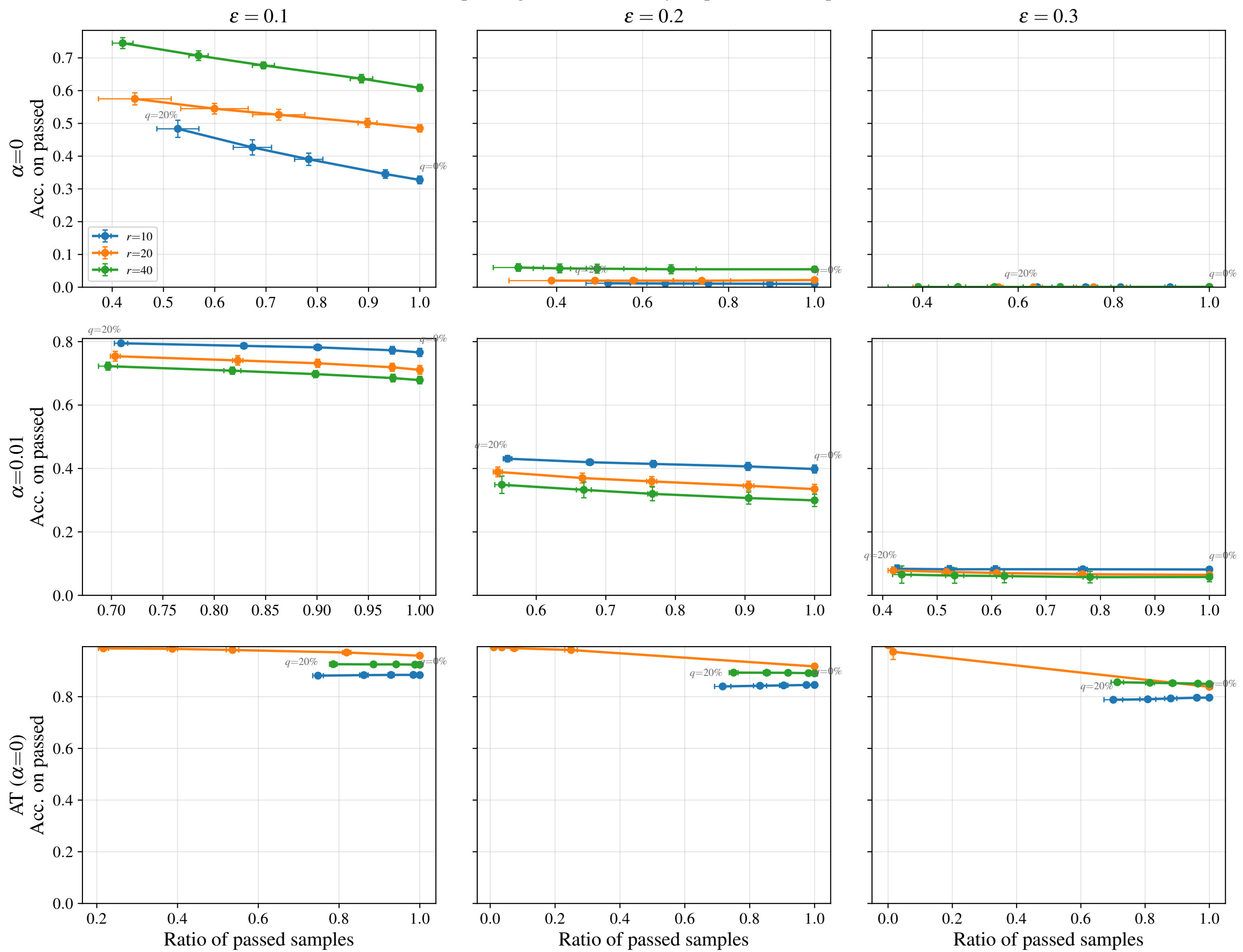
Detection operating curve — accuracy on passed vs ratio passed
